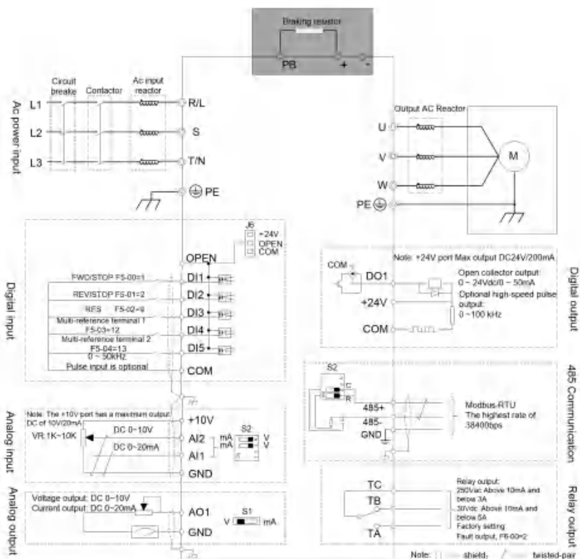
Fig. 3.1-1 Wiring diagram
