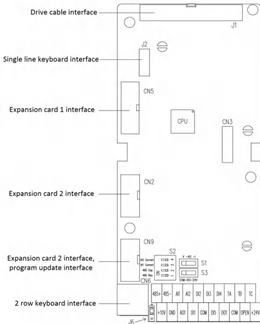
Fig. 3.2-1 Schematic diagram of control board layout
