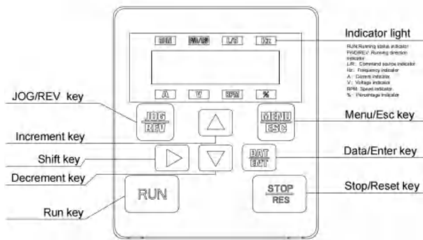
Fig.4.1-1 Control panel
